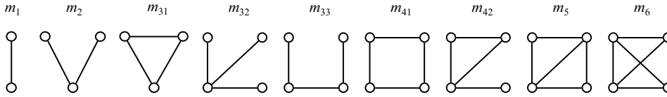
FIG 1. Correspondence between moments and motifs for K_4 .
